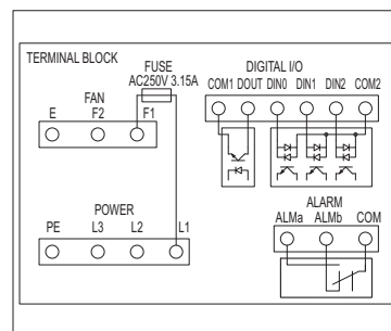
Wiring diagram
