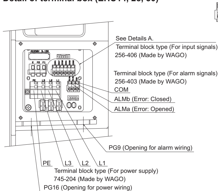
Wiring layout in the controller
